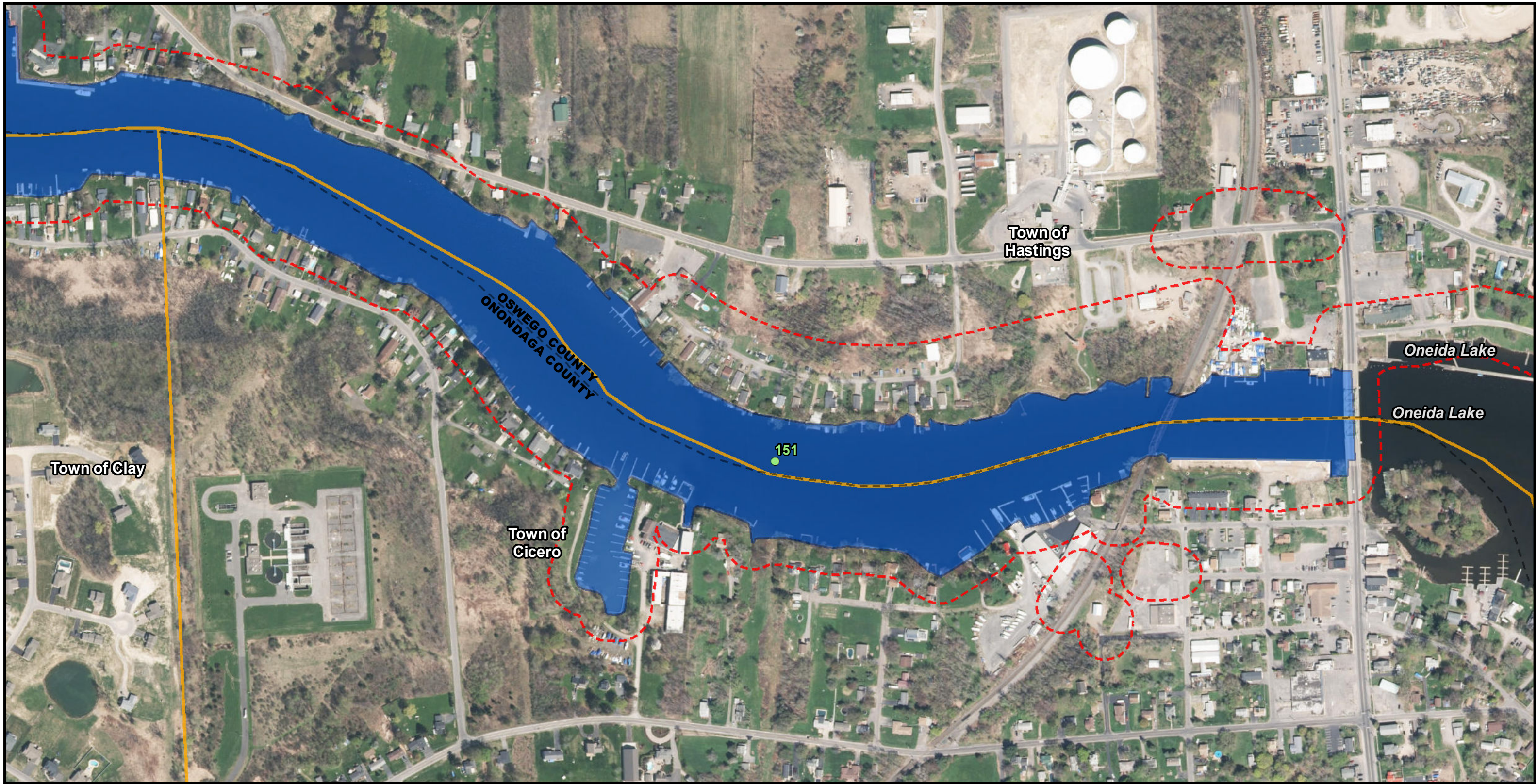
Figure 71F: Aquifers
